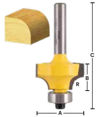
Rounding Over Bit
