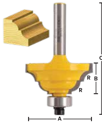
Classical Bit
